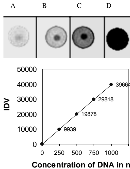
Fig. 4. Chromogenic Detection of bla gene. A, B, C and D correspond to 250, 500, and 750, 1000 ng of DNA blotted onto the membrane. Probe was used at the concentration of 50 ng/ml and was detected with the BCIP/NBT substrate as given in the materials and methods. The dots were scanned and the IDV, Integrated Density value (sum of all pixels) of each dot was measured automatically by the instrument after the background correction. Titration graph (dot intensity as IDV versus the DNA concentration spotted) was drawn and was found to be linear (intensity directly proportional to the amount of DNA used).
