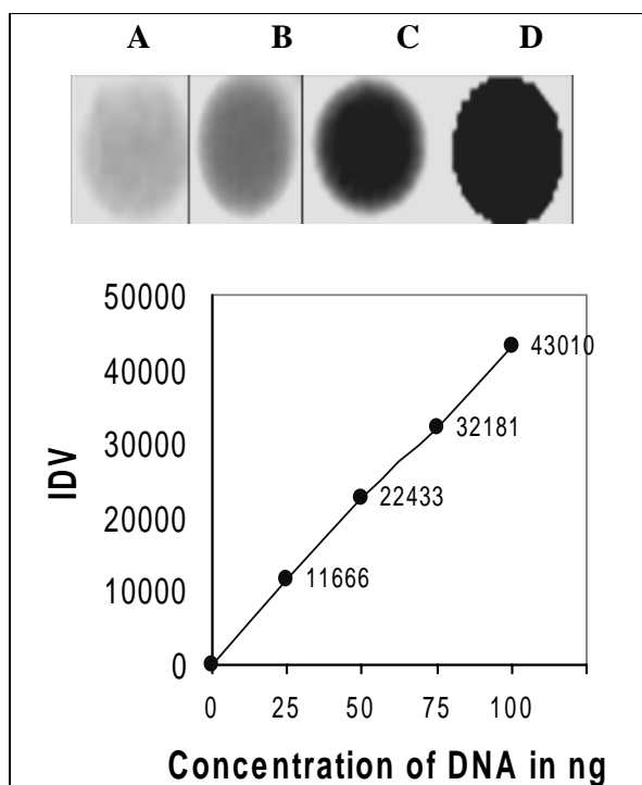
Fig. 5. Chemiluminescent Detection of aac(6) gene. A, B, C and D correspond to 25, 50, 75 and 100 ng of DNA blotted onto the membrane. Probe was used at the concentration of 50 ng/ml and was detected with the BCIP/NBT substrate as given in the materials and methods. The dots were scanned and the IDV, Integrated Density value (sum of all pixels) of each dot was measured automatically by the instrument after the background correction. Titration graph (dot intensity as IDV versus the DNA concentration spotted) was drawn and was found to be linear (intensity directly proportional to the amount of DNA used).
