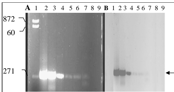
Fig. 2. PCR amplification and Southern Blot analysis of aac(6') gene in the clinical isolates of Pseudomonas aeruginosa A) 1.5in 1X TAE buffer containing 0.5 \mu\text{g/ml} ethidium bromide. Lane 1 DNA MI. wt. Marker ( \emptyset X 174 DNA- Hae III digest DNA). Lane 2 and 3 correspond to aminoglycoside positive samples 2 and 4 (1 \mu\text{g} of DNA). Lane 4 to 7 correspond to sample number 28 (aminoglycoside positive) and was loaded with 500, 50, 50 and 20 ng of PCR products respectively. Lane 8 was loaded with sample number 61 (aminoglycoside negative) Lane 9 was loaded with the reagent control (without template DNA). Arrow head showing the expected (260 bp) amplification product. B) Southern hybridization of the samples in gel A after transferring to Nylon membrane.
