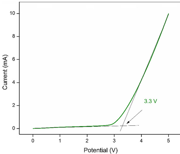
Fig. 10 Linear sweep voltammety of highest conducting polymer electrolyte
