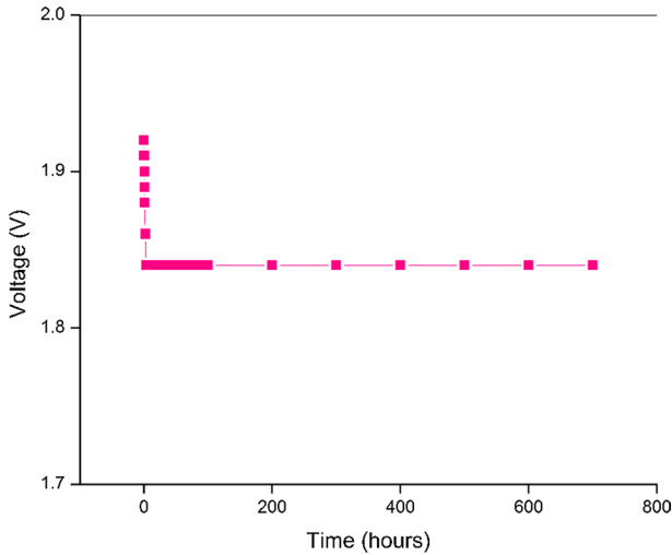
Fig. 12 Discharge characteristics of primary battery through 100 K \Omega (Mg | SPE | MnO 2 cathode)
